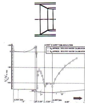
Figure 3 Halmi (1973) Pressure profile
