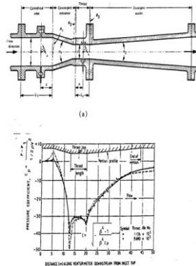
Figure 2 ASME Venturi Pressure Profile
