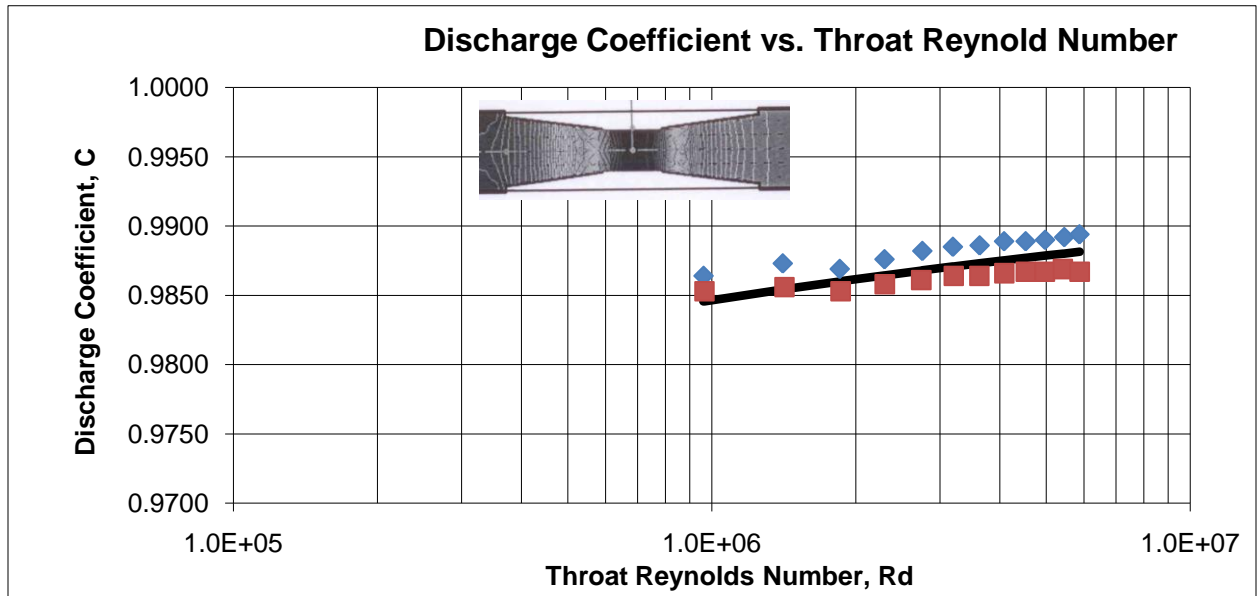
Figure 2 Discharge coefficients for AMITY's Bi Directional flowmeter.
