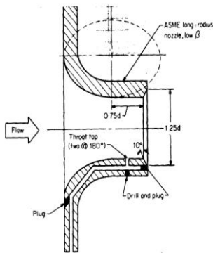
Figure 1 ASME PTC-6 Nozzle profile
