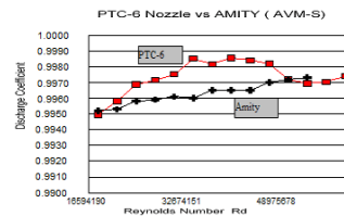
Figure 9 Comparison to PTC-6 data
