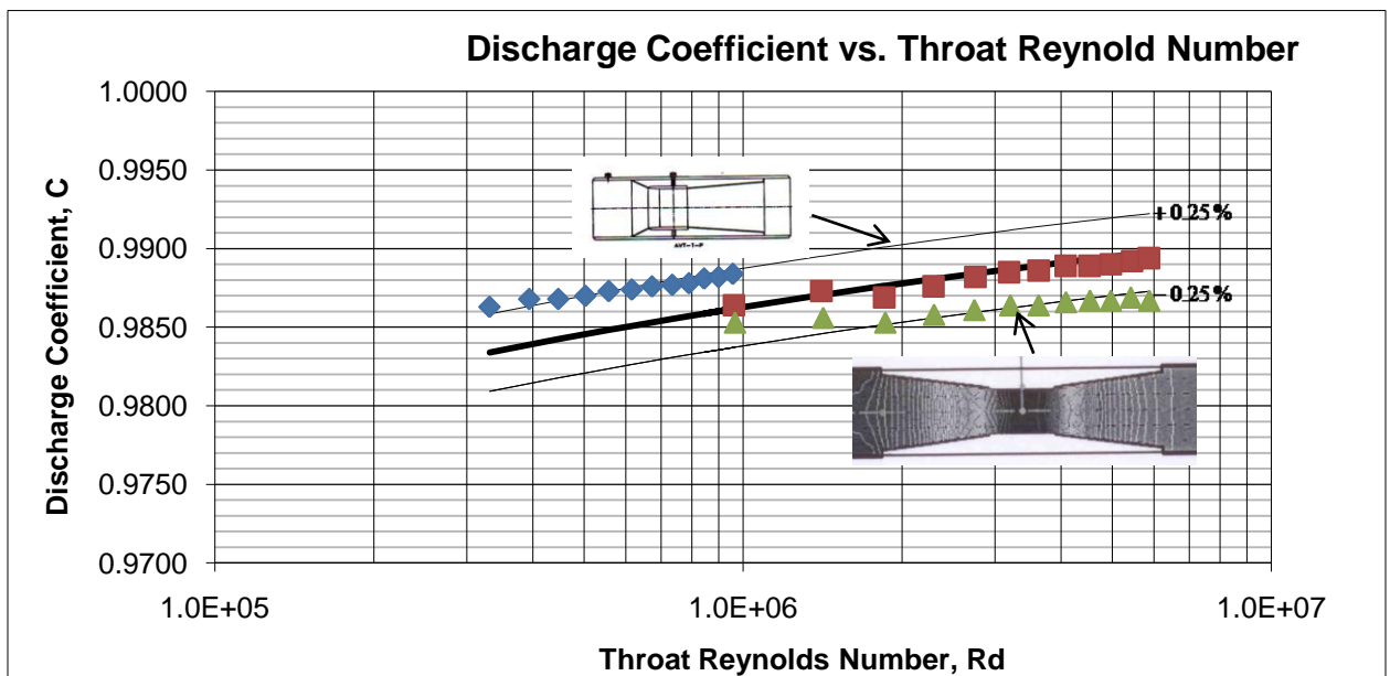
Figure 1 Discharge coefficient for AMITY's Bi Directional flowmeter.
