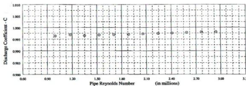
Figure 8 Typical Calibration Data
